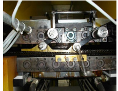
Centering slide bar top
